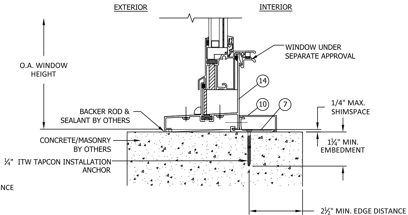
J 3 VERTICAL SECTION SILL - CONCRETE/MASONRY UNCLIPPED MULLION (2" EDGE CLIP)
