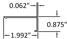
10 2" ANCHOR CLIP COVER 6063-T5
